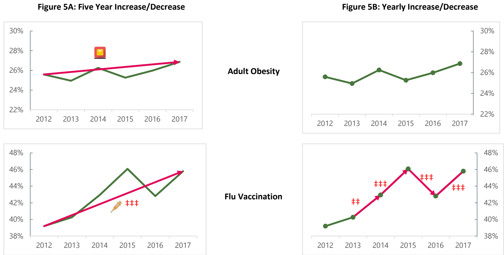
FIGURE 5: CHANGE IN SELECTED ANNUAL HEALTH INDICATORS, CT BRFSS 2012–2017
